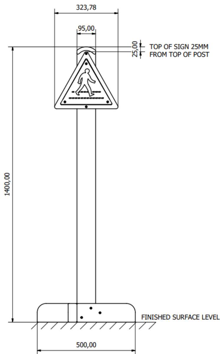
Side Elevation
