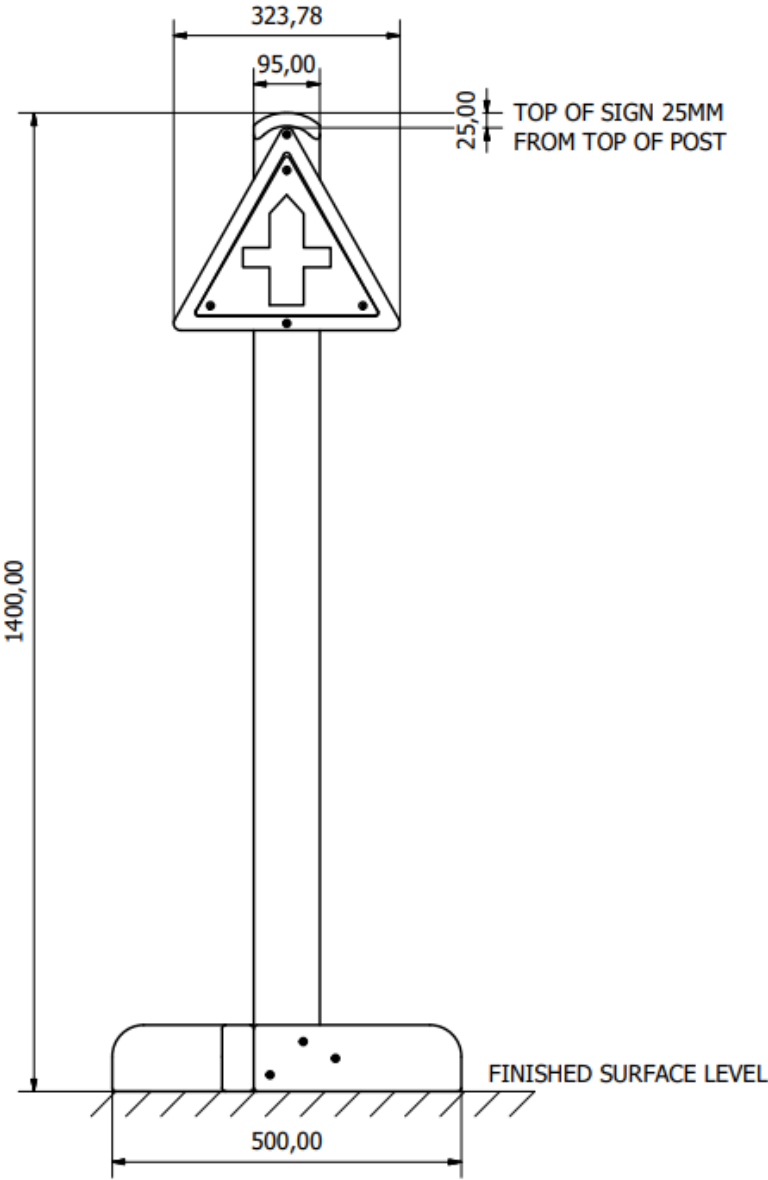
Side Elevation
