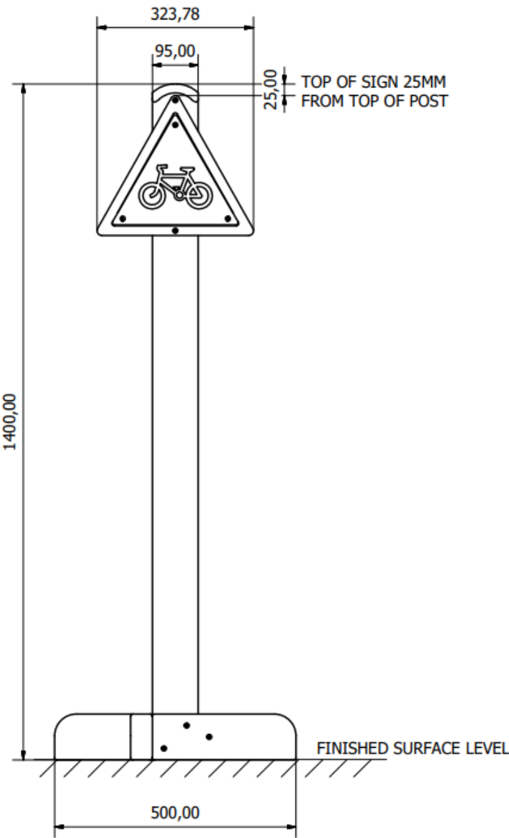
Side Elevation
