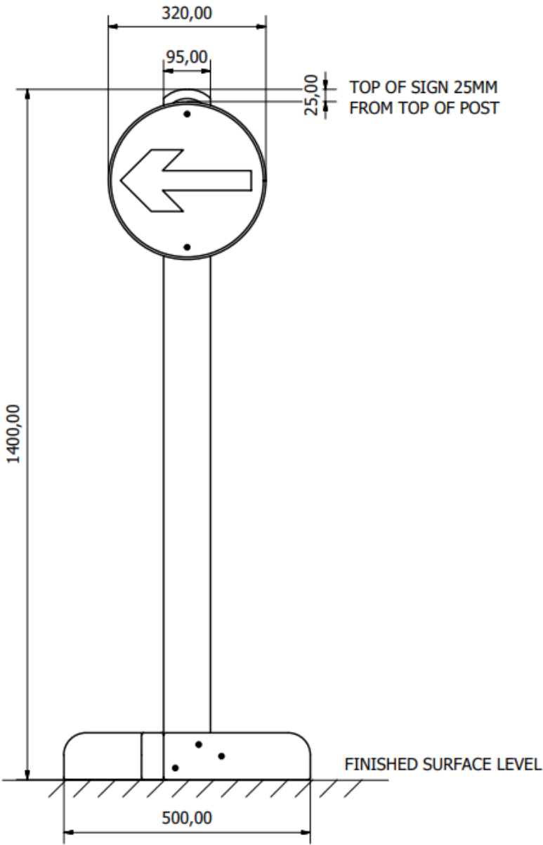
Side Elevation
