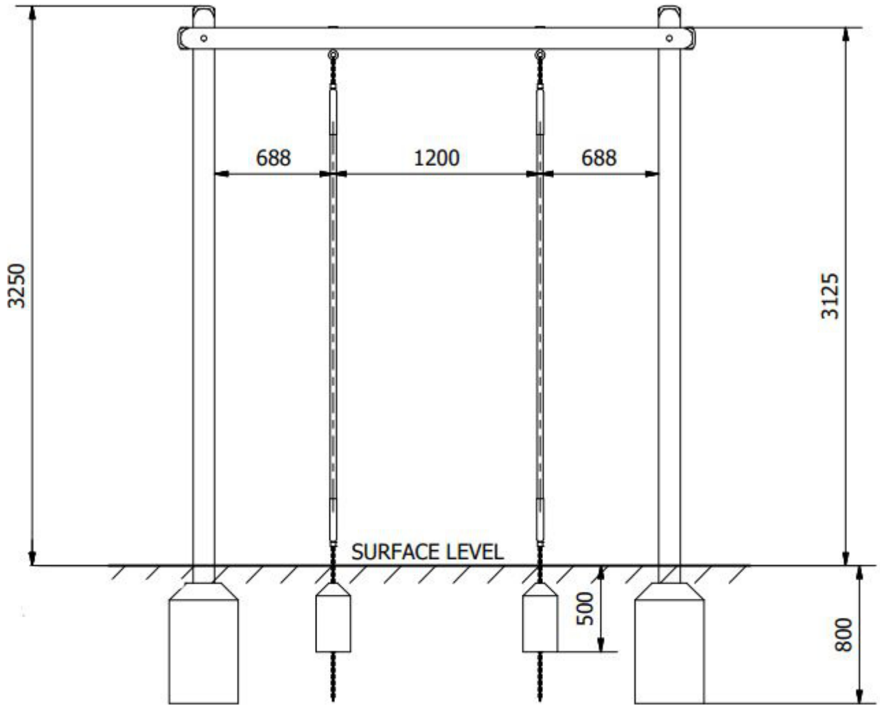
Side Elevation
