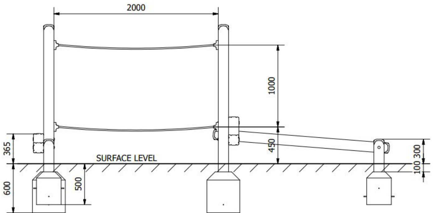
Side Elevation
