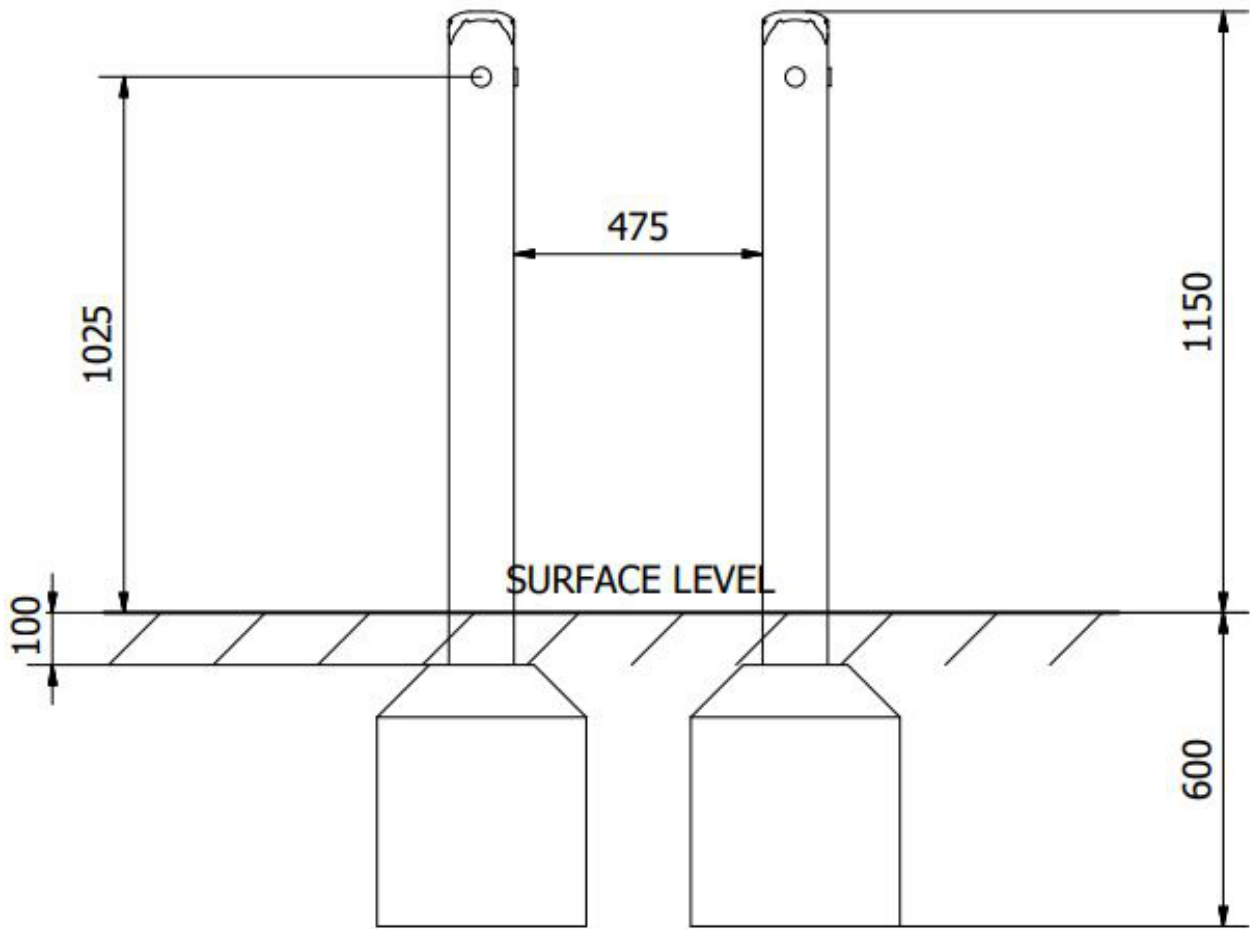
Side Elevation
