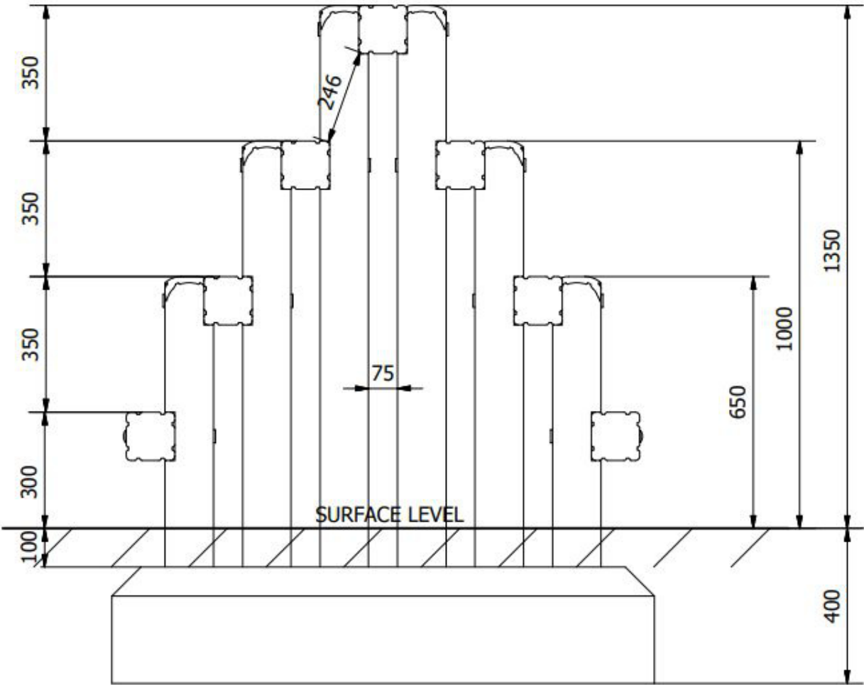
Side Elevation
