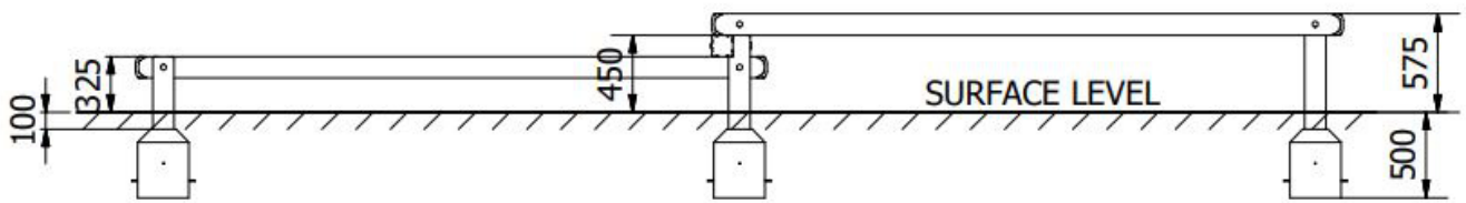
Side Elevation
